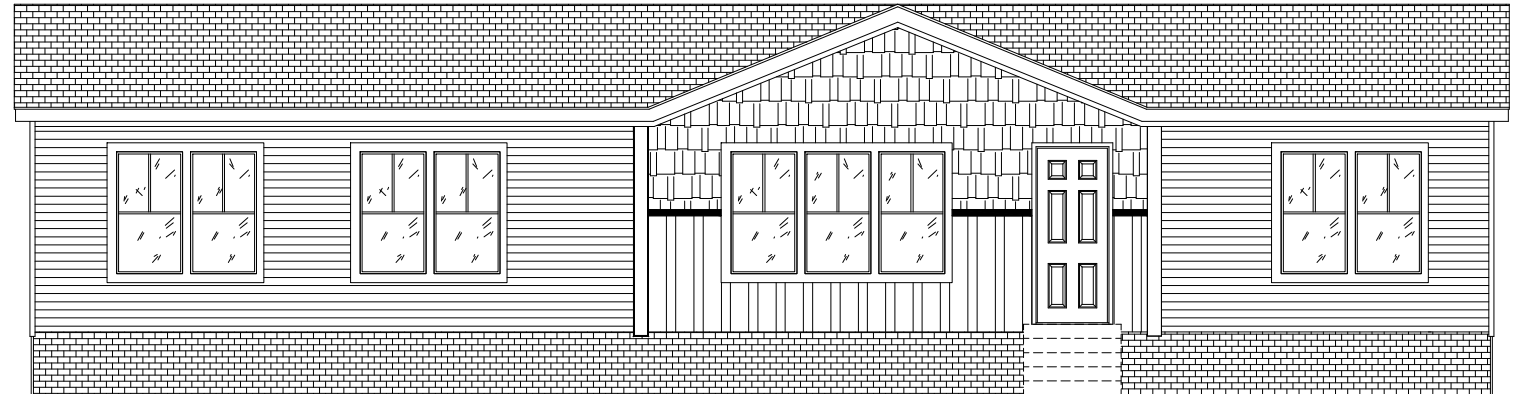
60'-4" FRONT ELEVATION
