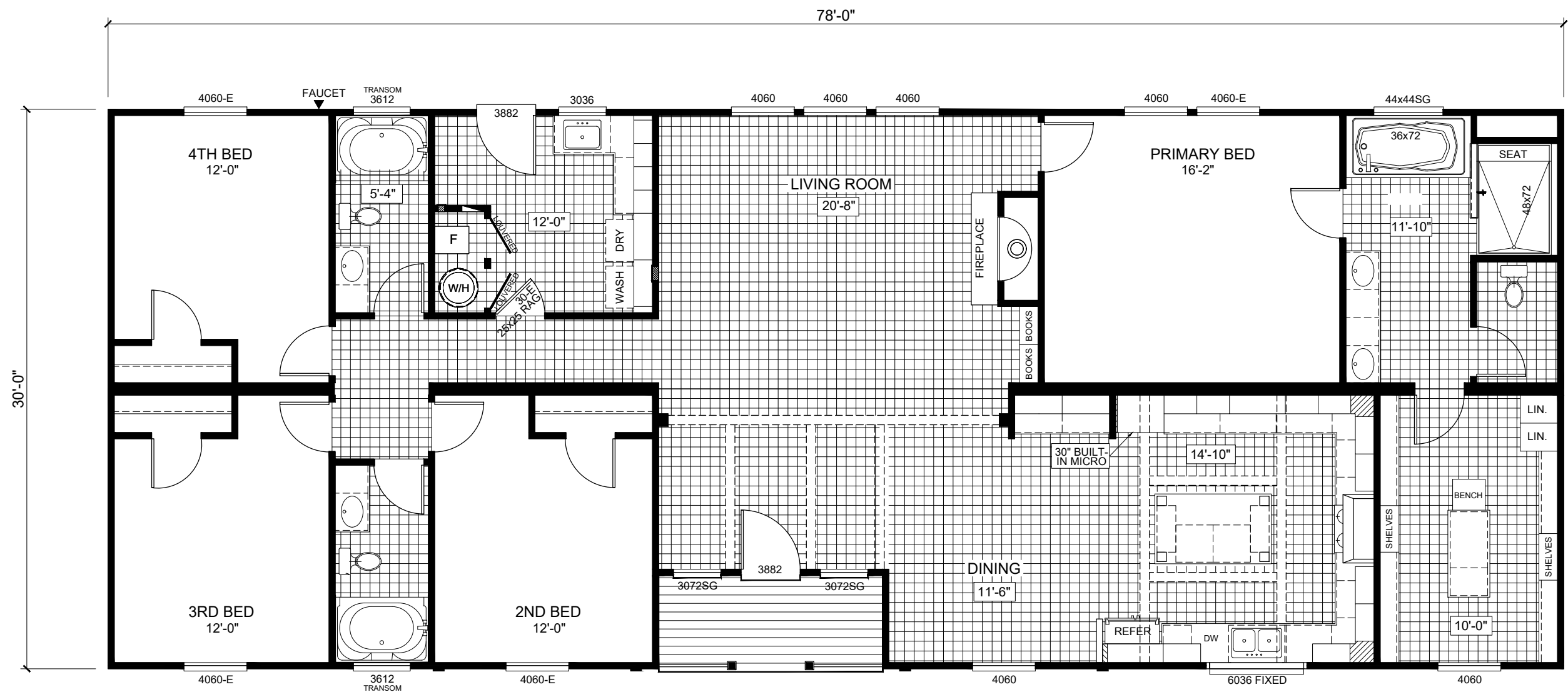
MODEL: 6753CAV The Bryant 3rd BATH OPTION 2X4 WALLS e-Built 4-BEDROOM / 2-BATH 32 x 78 (82) - Approx. 2340 Sq. Ft.
