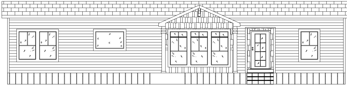
FRONT ELEVATION
