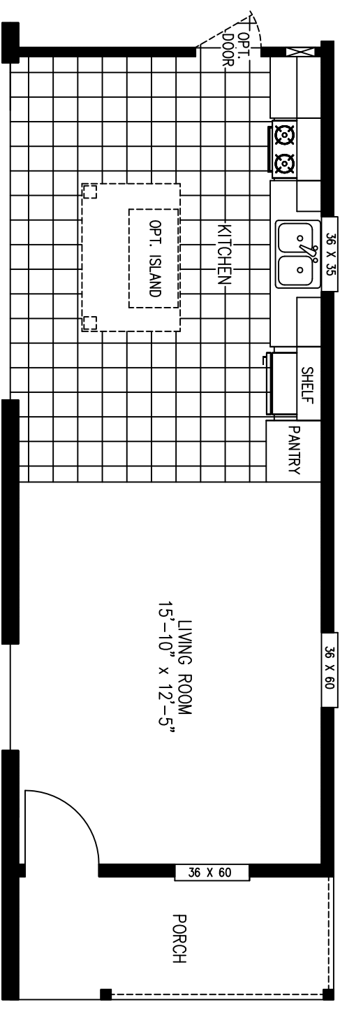
END ENTRY OPTION W/ 5' PORCH
