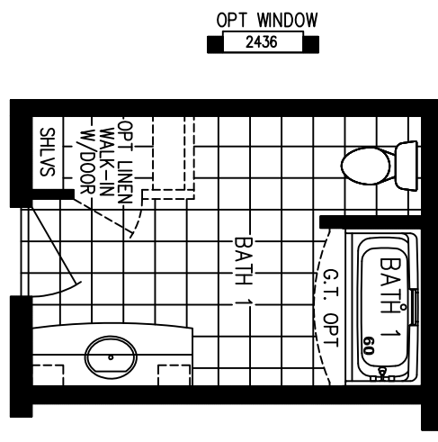
OPTIONAL BATH VANITY W/ DUAL TOWERS
