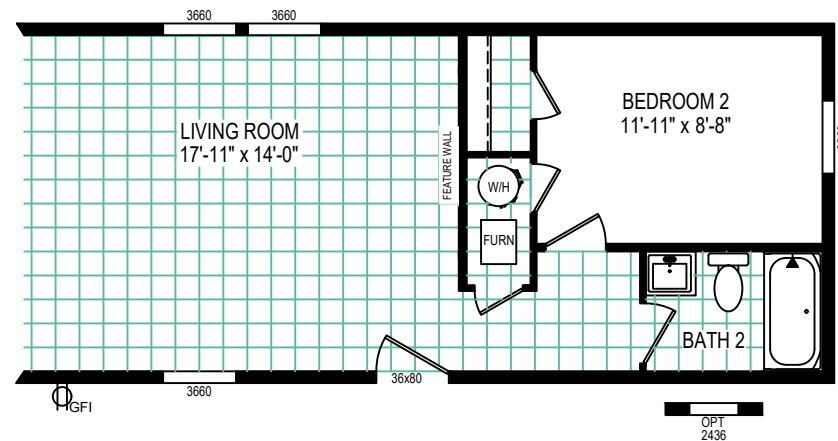
2-BEDROOM OPTION
