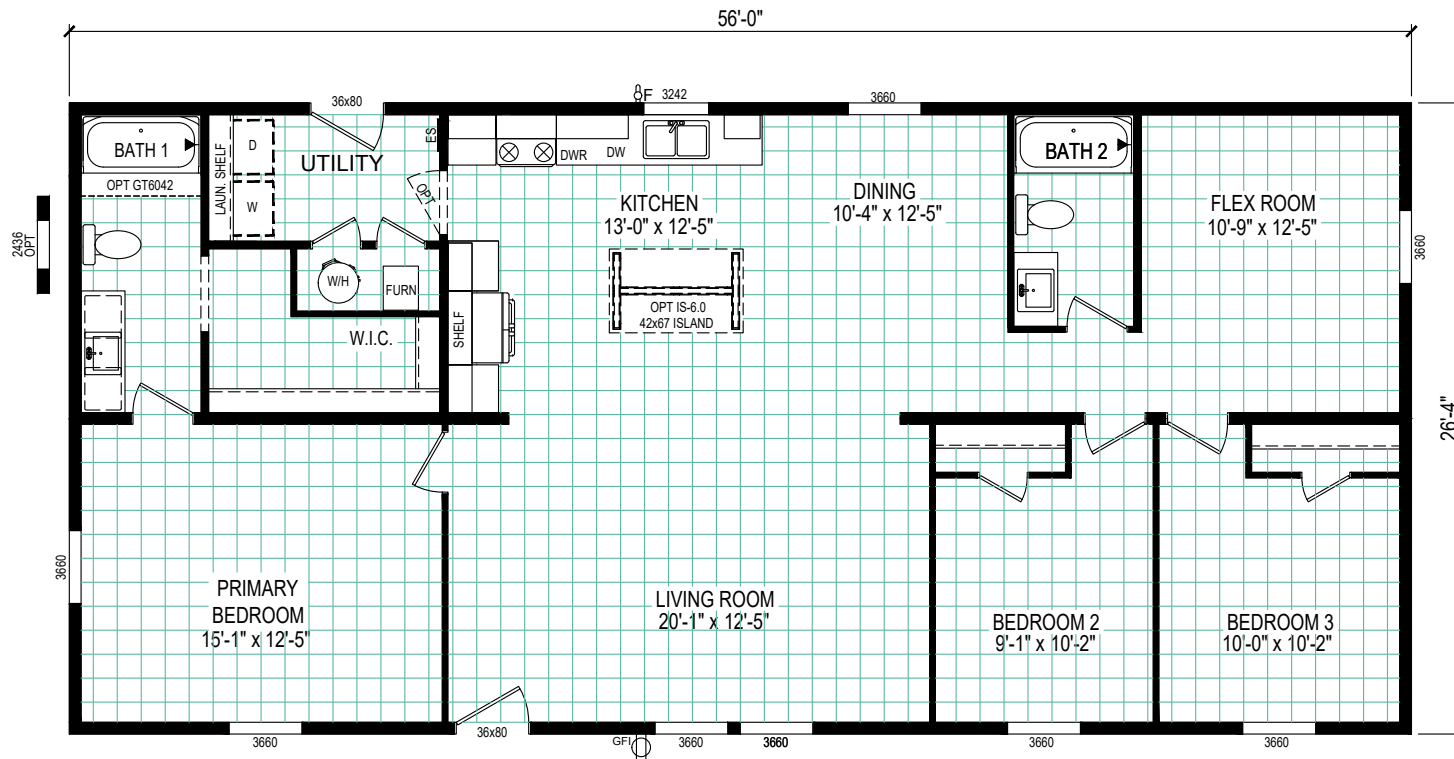
Compass 56 Model: 5628-CC52RE 1475 Square Feet - 3 Bed / 2 Bath
