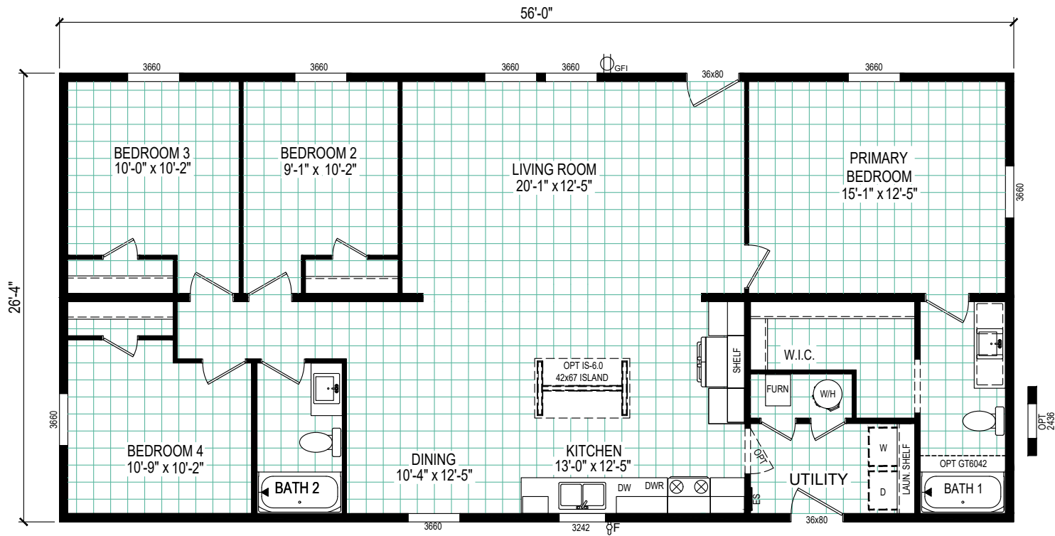
Compass 56 Model: 5628-CC52RS-4BR 1475 Square Feet - 3 Bed / 2 Bath
