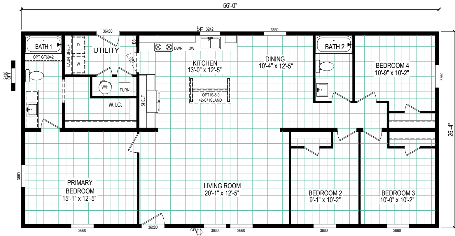
Compass 56 Model: 5628-CC52RE-4BR 1475 Square Feet - 3 Bed / 2 Bath
