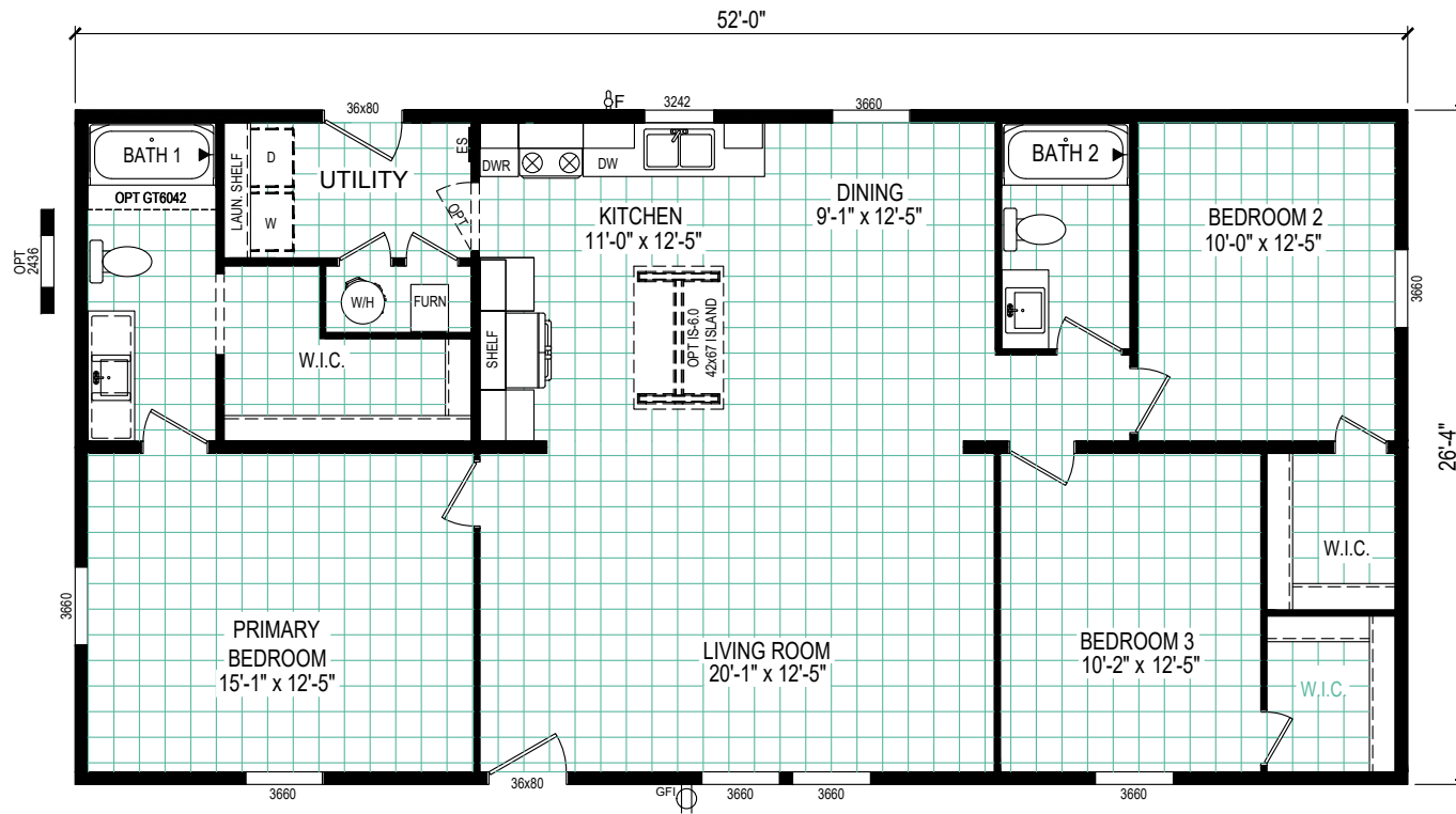
Pillar 52 Model 5228-CC51RE 1369 Square Feet - 3 Bed / 2 Bath
