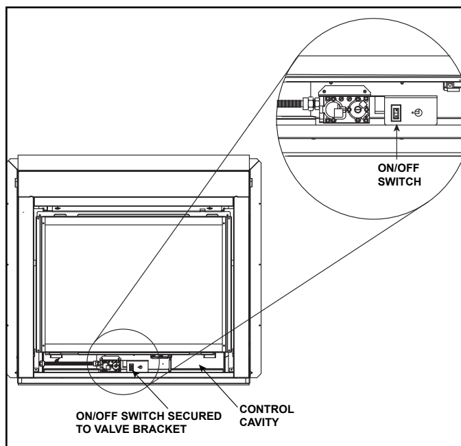
Figure 3.6 ON/OFF Switch Location
