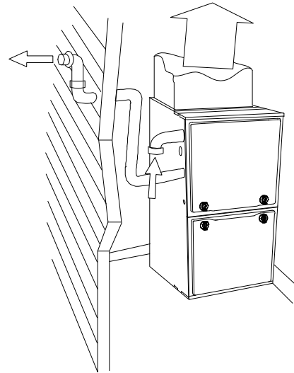
Figure 3 Interior Combustion – Air Pipe
