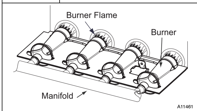
Figure 5 Burner Flame Adjustment
