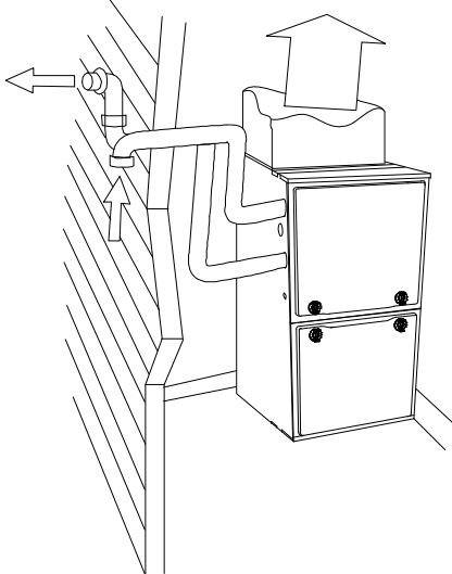
Figure 2 Exterior Vent Pipes
