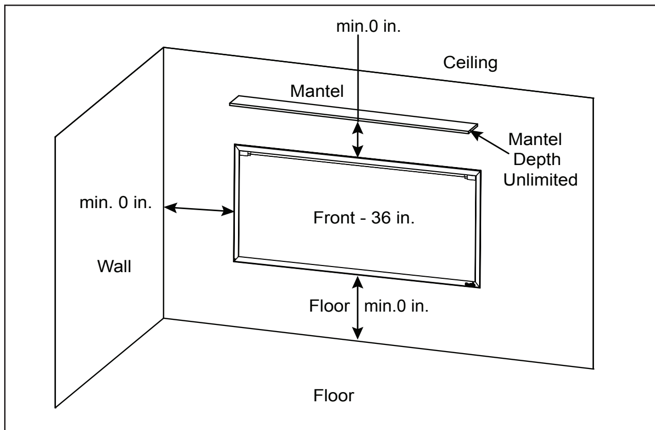
Figure 3.2 Location and Clearances Requirements
